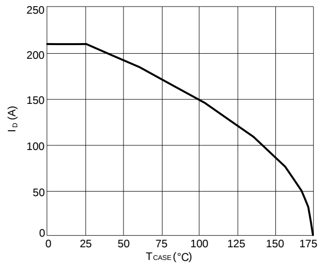
Figure 8: Current De-rating
