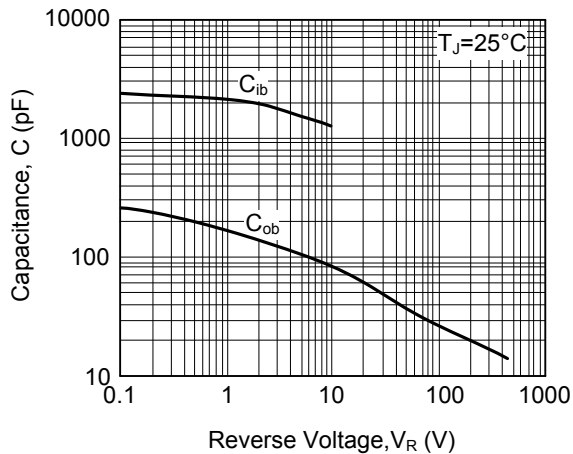
Figure 6. Capacitance
