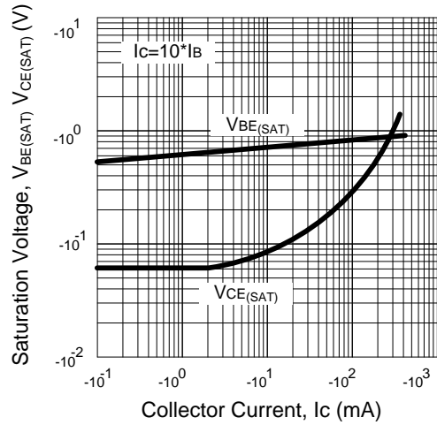
Fig.4 Saturation Voltage
